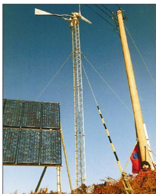
Fig. 4 – Power system
