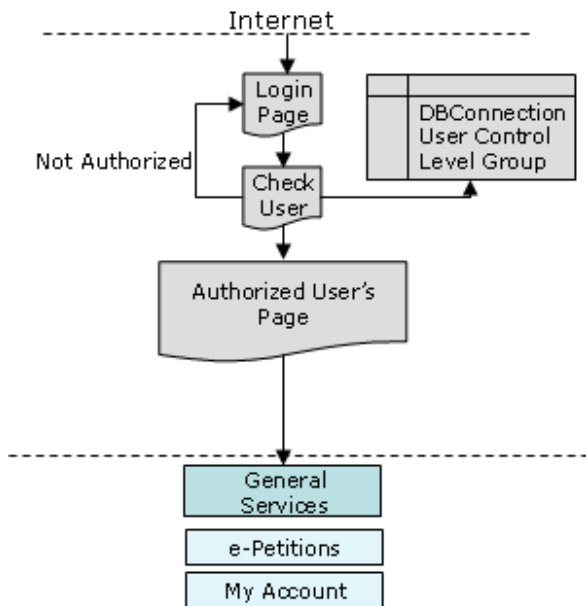
Figure 5 – Tools of the Registered User's Environment
