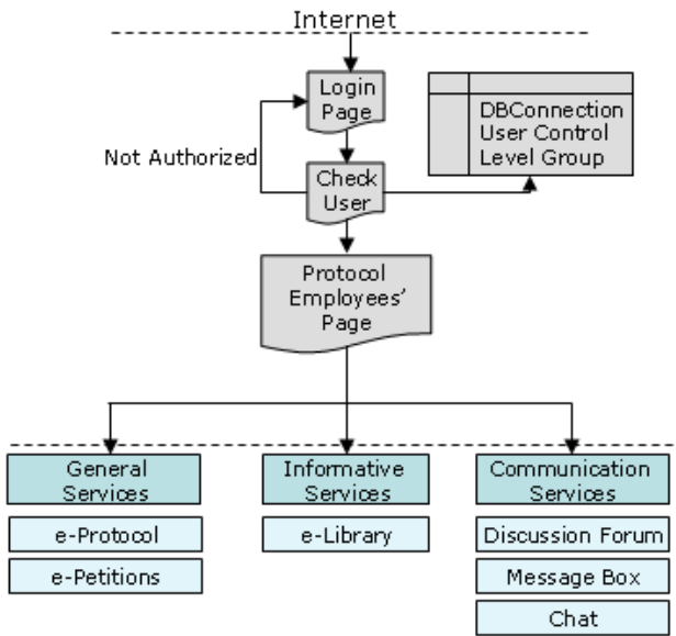
Figure 4 – Tools of the Protocol Administrator Environment
