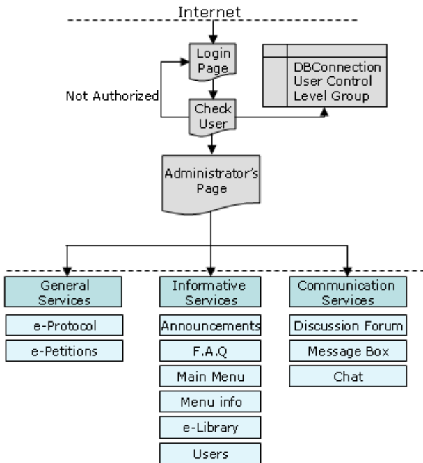
Figure 2 - Administration Tools
