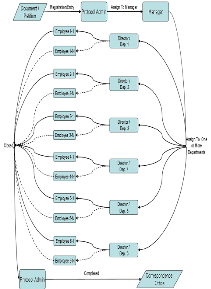
Figure 7 – e-Protocol Chain
