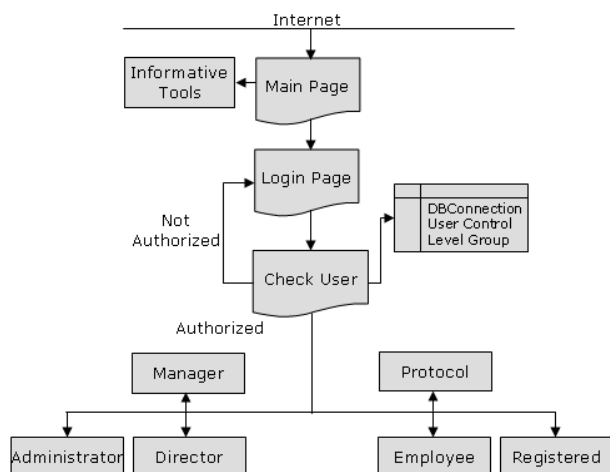
Figure 1 – User Levels
